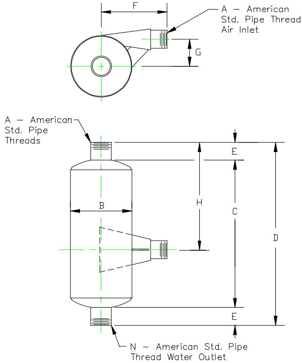
Sizes 1 Through 3 1/2
