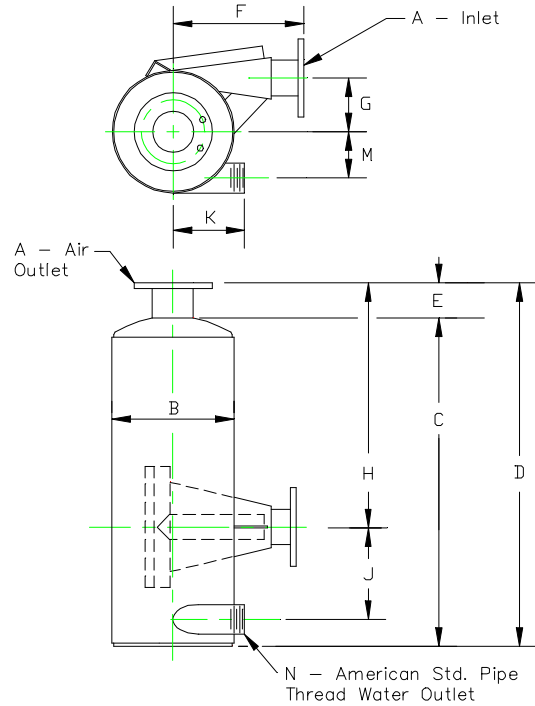
Sizes 4 Through 16
