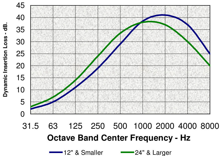
Typical Performance
